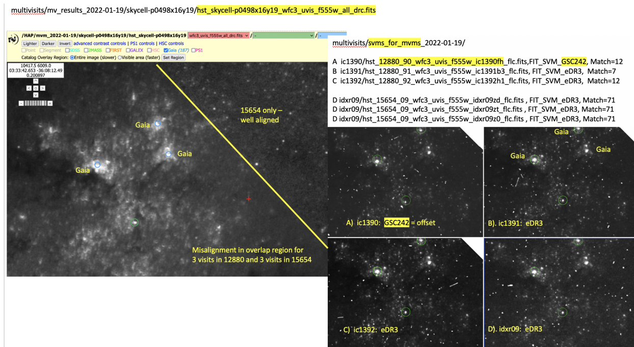
Fig. 7: All the WFC3/UVIS F555W exposures that overlap SkyCell p0498x16y19 illustrating how misalignment between visits can result in ‘blurred’ sources in region of overlap. [Image courtesy of J. Mack (STScI/ACS Instrument team)].
