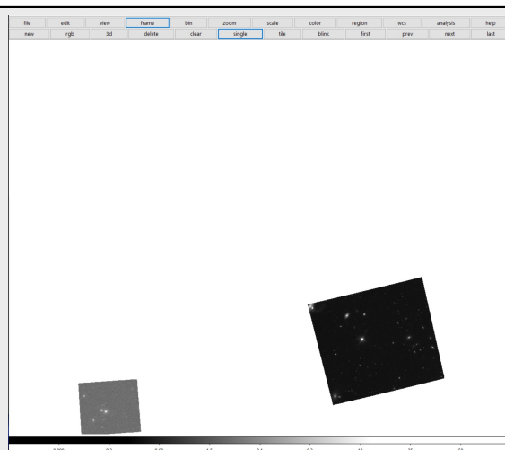
Fig. 6: All the WFC3/IR F105W exposures that overlap SkyCell p1889x07y19 .
